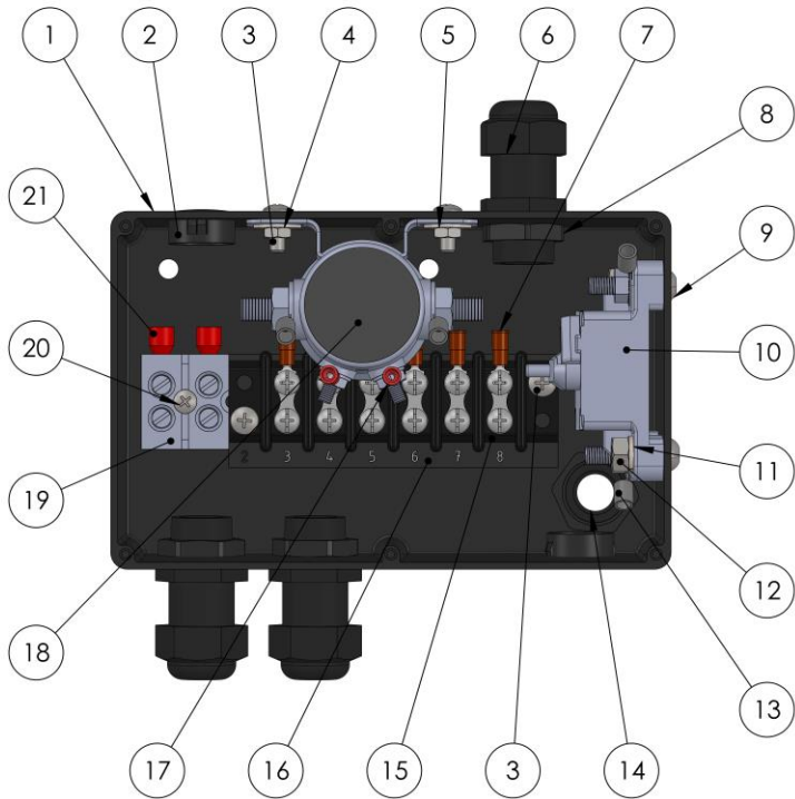
Figure 15: 503-019 ELECTRICAL BOX
