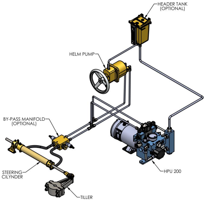
Figure 19: Typical System Arrangement, Closed Loop
