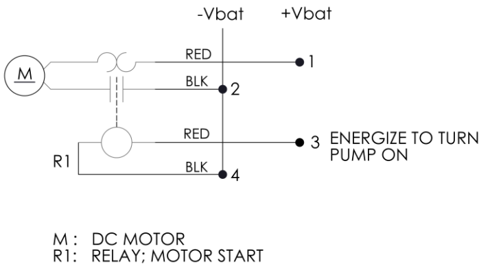
Figure 6: HPU200 DC Motor Wiring Diagram
