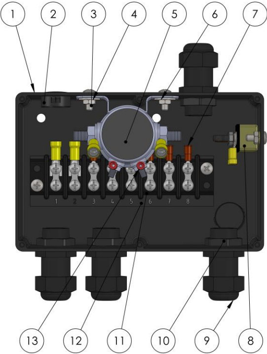
Figure 16: 503-020 ELECTRICAL BOX
