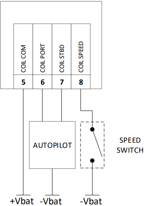
Figure 10: HPU200 Autopilot Wiring Diagram, Common Positive
