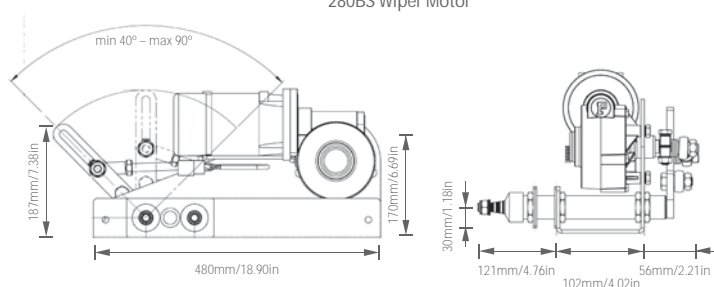
280BS Wiper Motor
