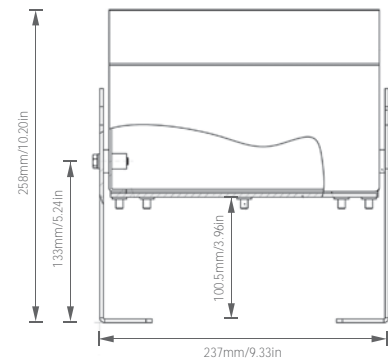
223XBD Wiper Motor
