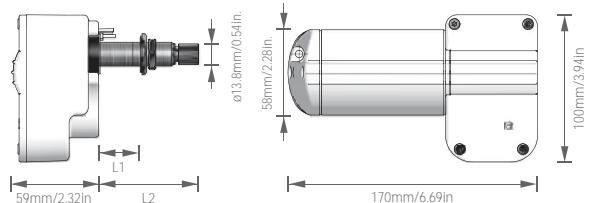
W12 Series Motor
