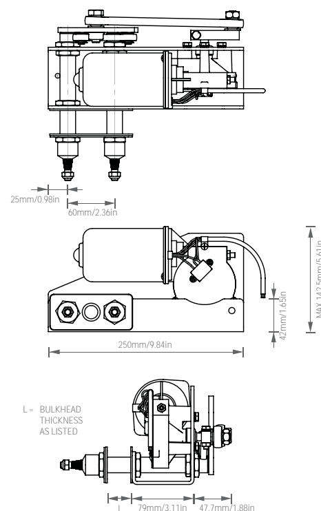
255BS Wiper Motor
