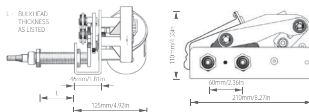
W38 Series Motor
